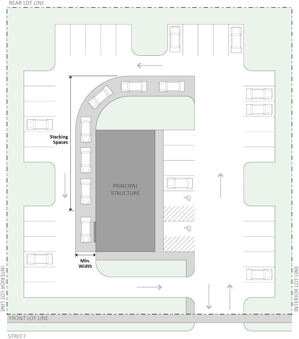
Figure 10.07.1 Stacking Spaces
